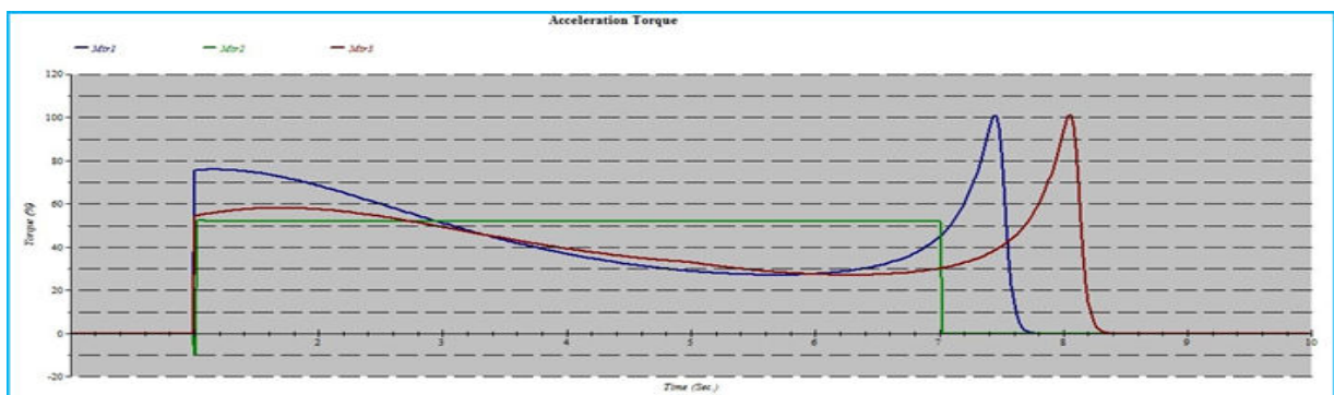
Figure 6 % of acceleration torque – time
