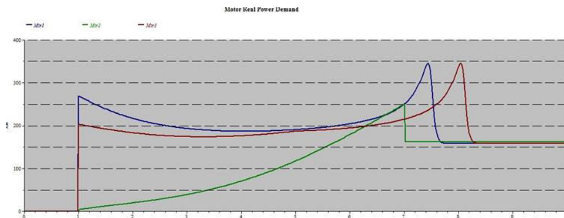
Figure 10 Motor real power demand – time
