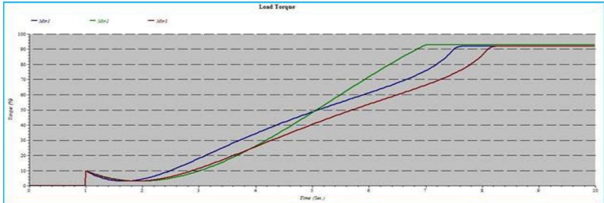
Figure 3 % of load torque – time
