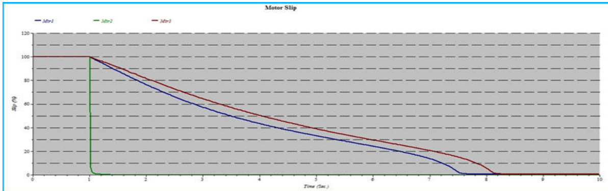
Figure 7 % of motor slip – time
