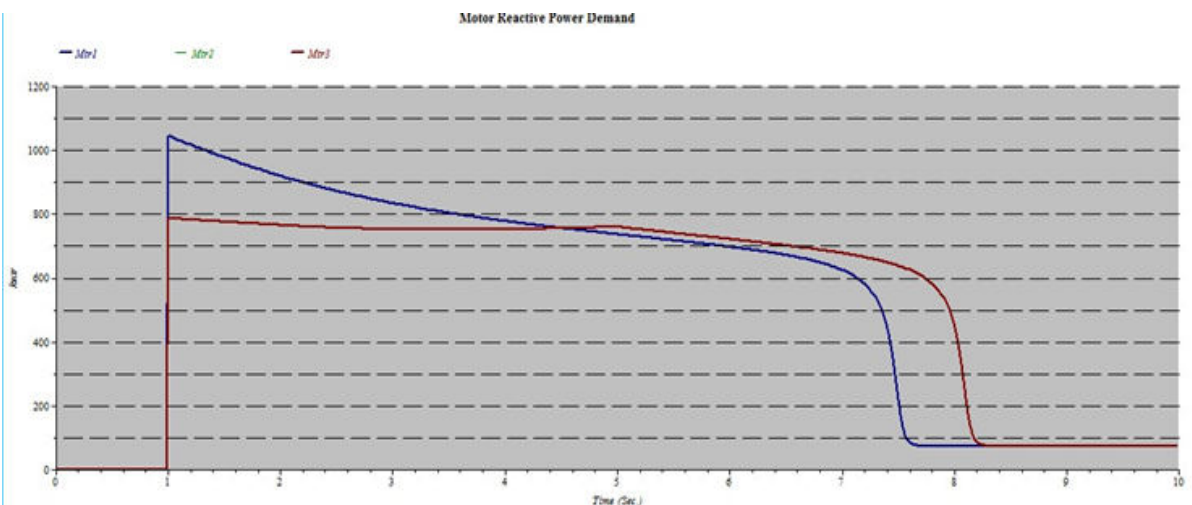
Figure 9 Motor reactive power demand – time
