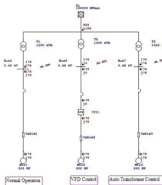
Figure 1 Load flow analysis of test model
