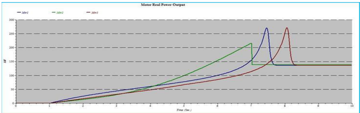
Figure 8 Motor real power output – time
